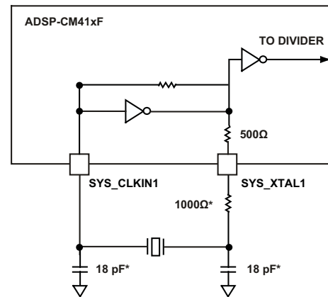
Figure 16. External Crystal Connection for CLKIN0
