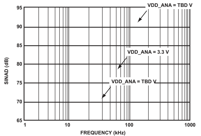
Figure 24. SINAD vs. Frequency, 0 to 1.5 V
