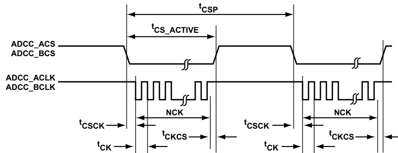
Figure 71. ADC Timing
