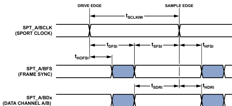
Figure 43. Serial Ports—Data Receive/Internal Clock
