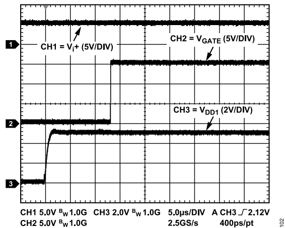
Figure 6. Typical V_{DD1} Startup to Output Valid
