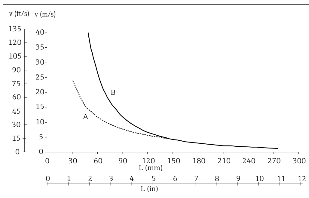
9 Permitted flow velocities, thermowell diameter 6.35 mm (1/4 in)
