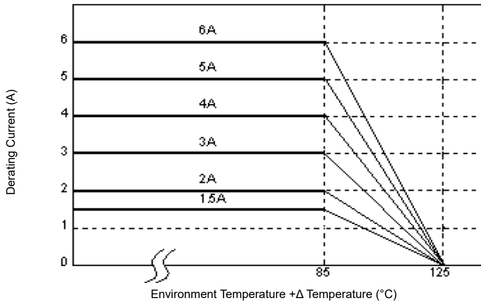
Derating Curve
