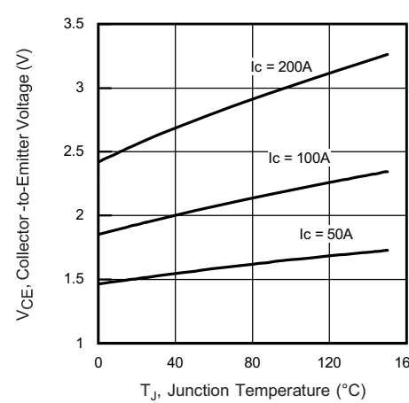
Fig. 4 - Typical Collector to Emitter Voltage vs. Junction Temperature
