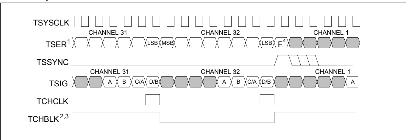
Figure 35-10. Transmit-Side 2.048MHz Boundary Timing (Elastic Store Enabled)
