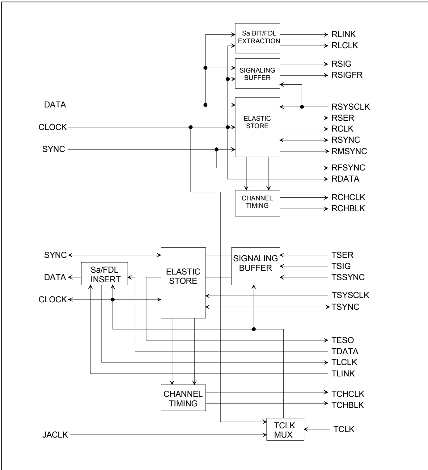
Figure 3-4. Backplane Interface
