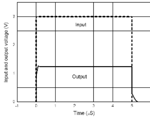
Fig. 12: Pulse Response
