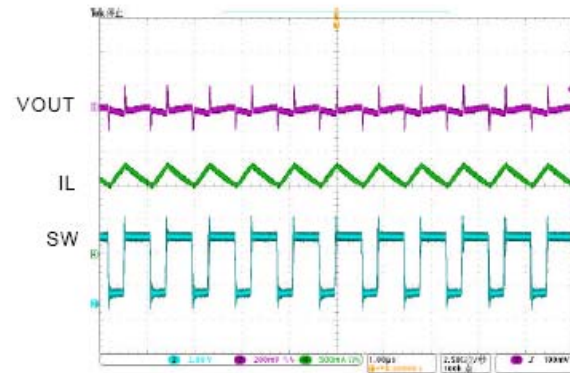
8. Switching Waveform
