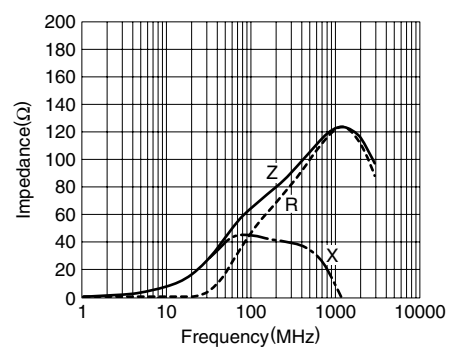
MZA3216Y600B
