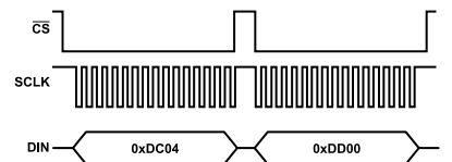
Figure 34. SPI Sequence for Writing 0x0004 to FILT_CTRL
