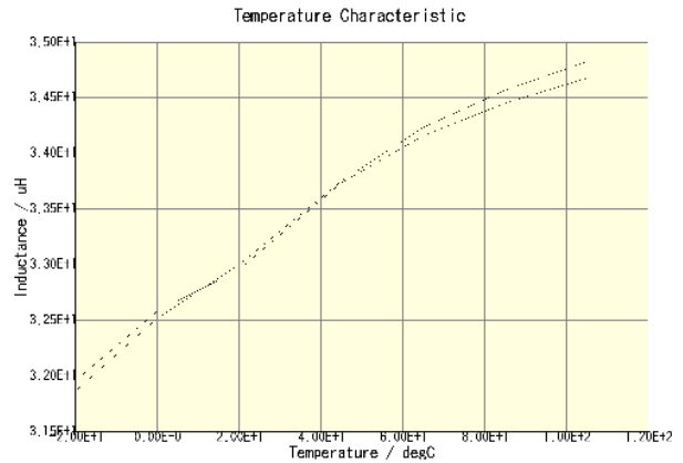
CLF10040T-330M-CA(DC = 0A)
