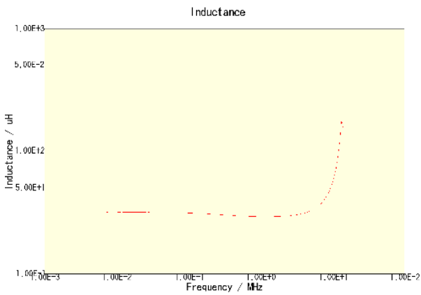
CLF10040T-330M-CA
