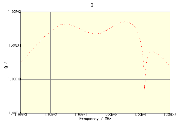
CLF10040T-330M-CA
