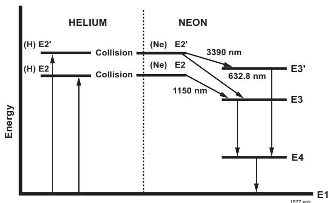
Figure 11. Energy Levels of Gas Laser (Detail)
