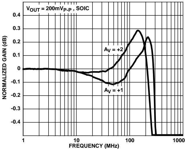
FIGURE 14. GAIN FLATNESS
