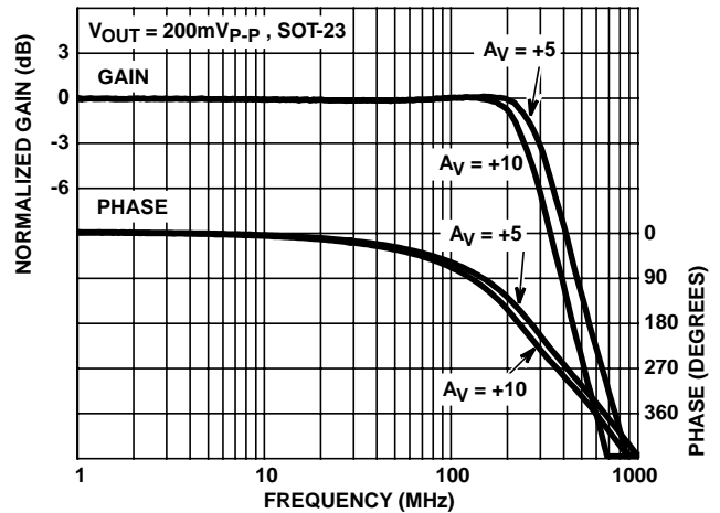
FIGURE 17. FREQUENCY RESPONSE
