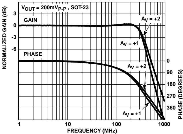
FIGURE 16. FREQUENCY RESPONSE
