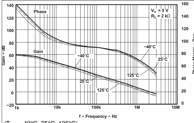
(TA = -40°C, 25°C, 125°C) Figure 21. Gain and Phase Margin vs Frequency
