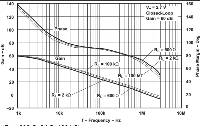
(RL = 600 Ohm, 2 kOhm, 100 kOhm) Figure 22. Gain and Phase Margin vs Frequency
