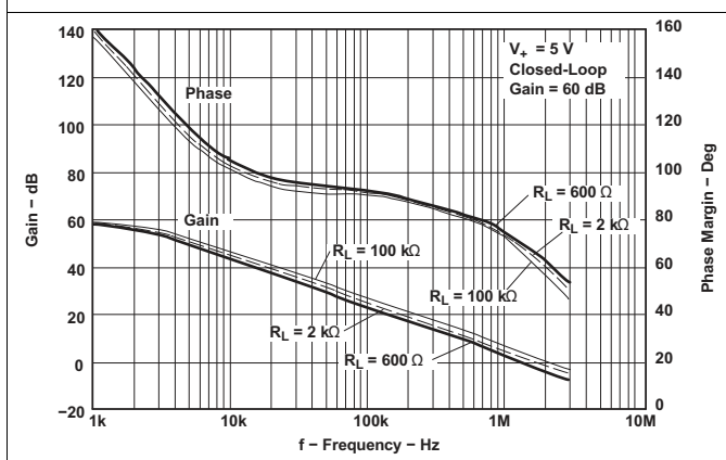
(RL = 600 Ohm, 2 kOhm, 100 kOhm) Figure 23. Gain and Phase Margin vs Frequency
