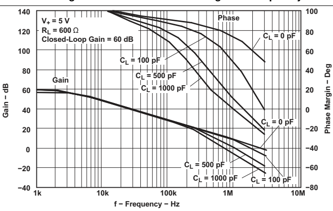
(CL = 0 pF, 100 pF, 500 pF, 1000 pF) Figure 24. Gain and Phase Margin vs Frequency
