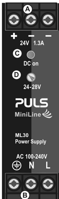
Fig. 10-1 Front side
