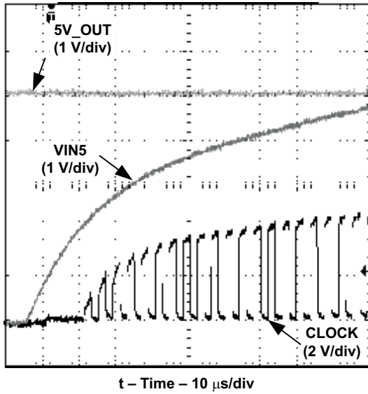
Figure 15. Clock Startup
