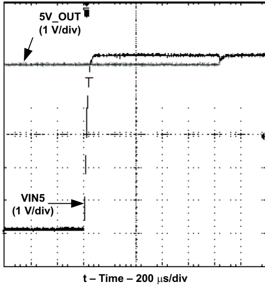
Figure 11. 5.0-V Switchover
