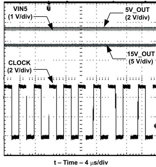
Figure 16. Clock Steady
