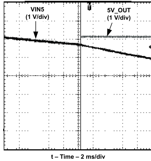
Figure 12. 5.0-V Switchover
