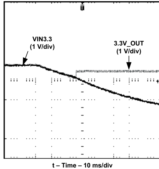
Figure 14. 3.3-V Switchover
