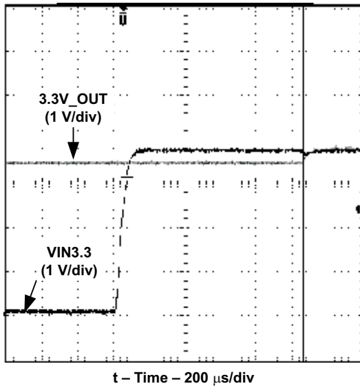
Figure 13. 3.3-V Switchover
