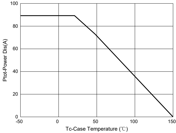
Fig. 9 - Power dissipation
