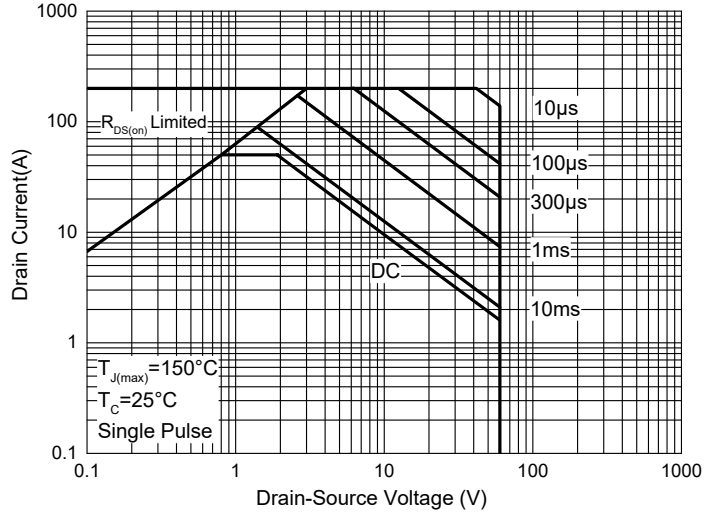
Fig. 10 - Safe Operation Area
