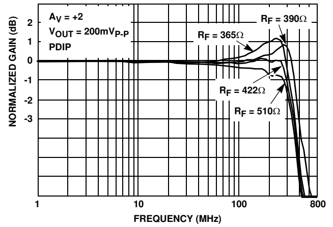
FIGURE 31. FREQUENCY RESPONSE vs FEEDBACK RESISTOR
