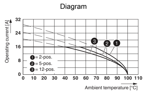
Type: FKC 2,5 HC/...-STF with MSTB 2,5 HC/...-GF
