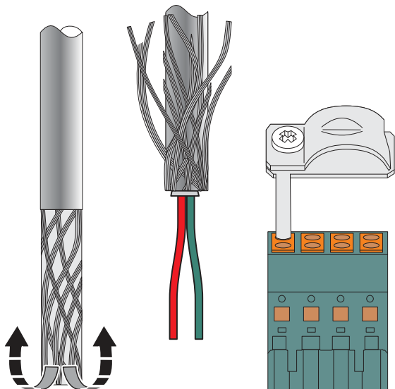
Figure 6 Push the braided shield back
