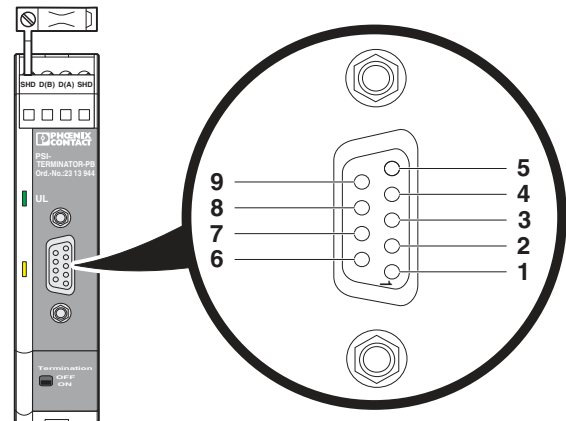
Figure 2 D-SUB, programming interface
