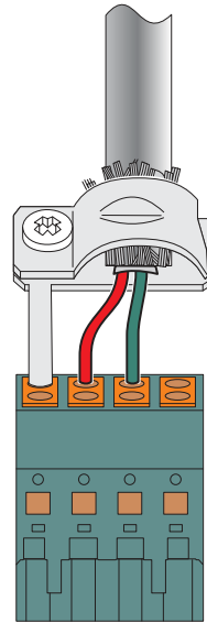
Figure 7 Connecting cables with a shield clip
