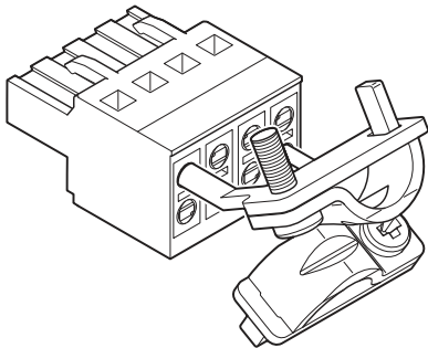
Figure 5 Install shield clip
