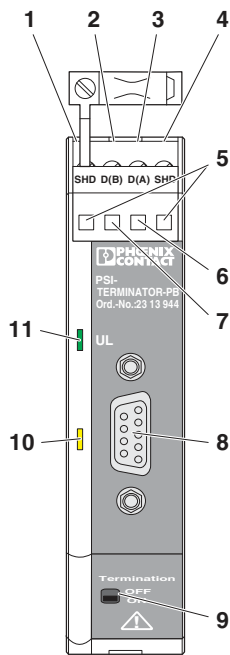
Figure 1 Function elements
