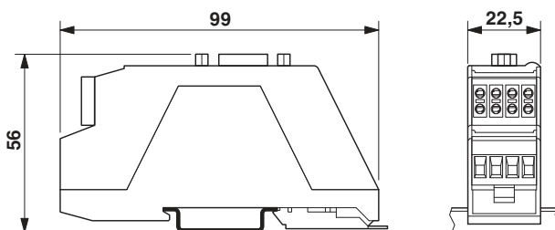
Figure 4 Dimensions
