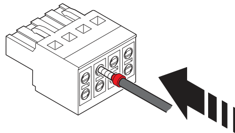
Figure 8 Install signal cable
