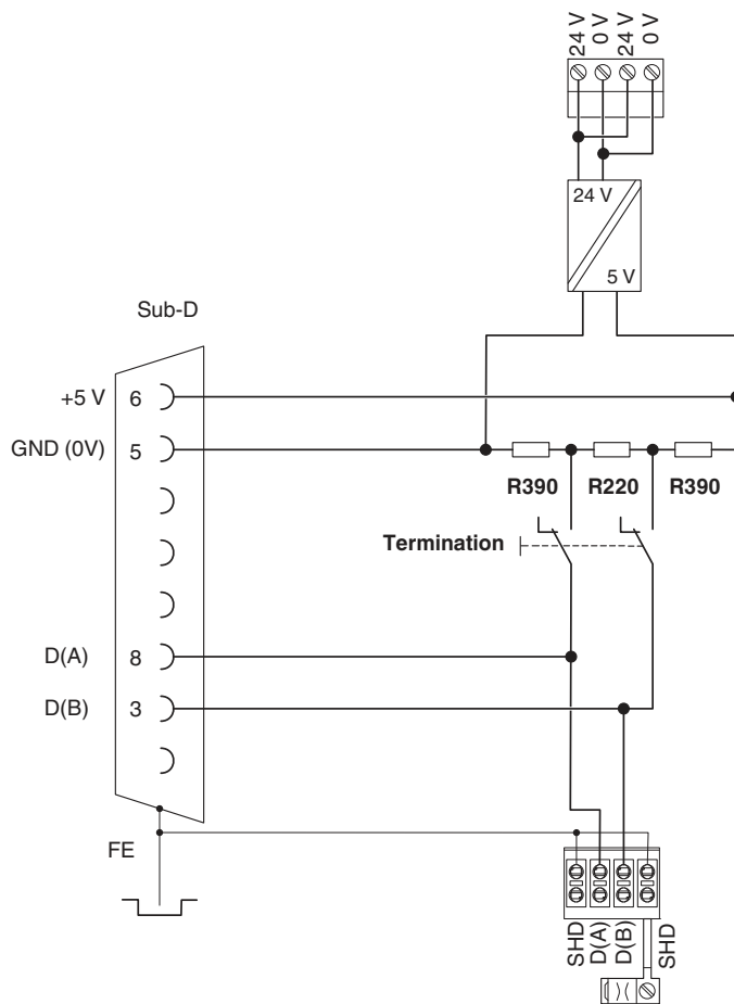
Figure 3 Block diagram
