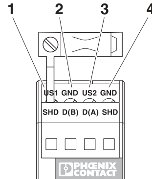
Figure 10 Power supply
