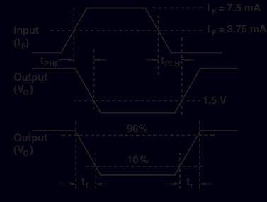
Fig. 20 Test Circuit and Waveforms for t_{PLH} , t_{PHL} , t_r and t_f
