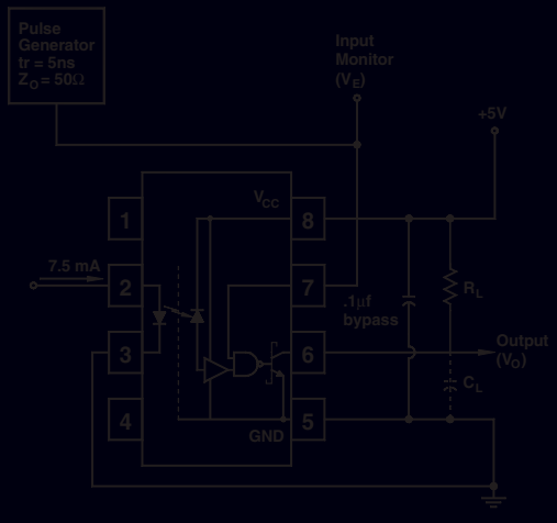
Fig. 21 Test Circuit t_{EHL} and t_{ELH}
