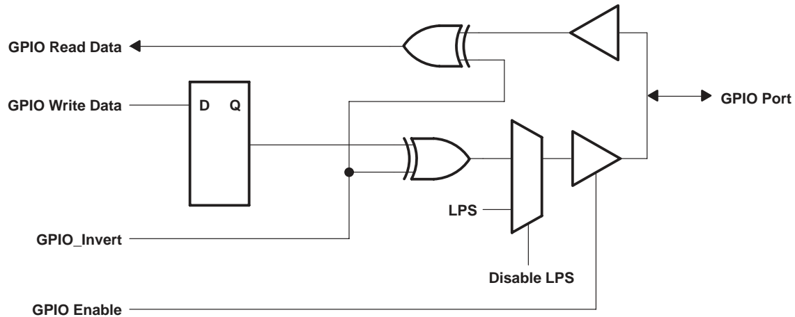
Figure 23. LPS/GPIO1
