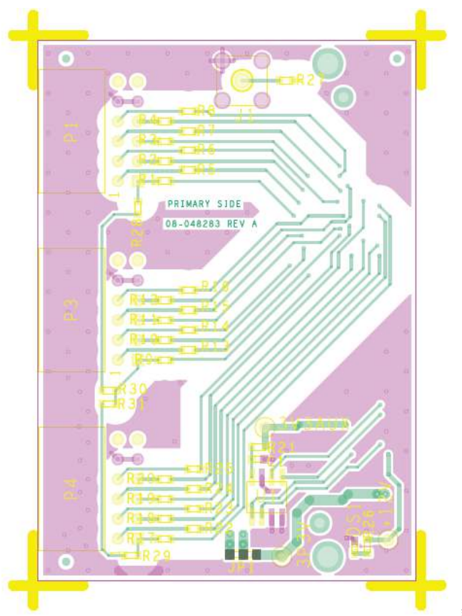
Figure 33. EVAL-PMD-IB1Z, Top Layer
