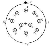
Contact Layout
