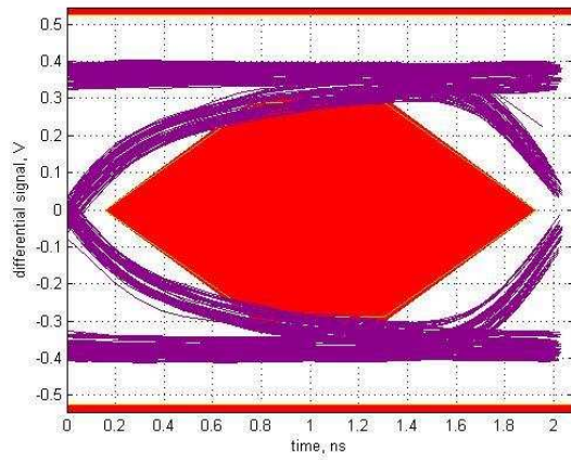
Figure 2. USB2.0 HS Eye diagram, Host far-end with 2m cable post-channel loss without TUSB215-Q1
