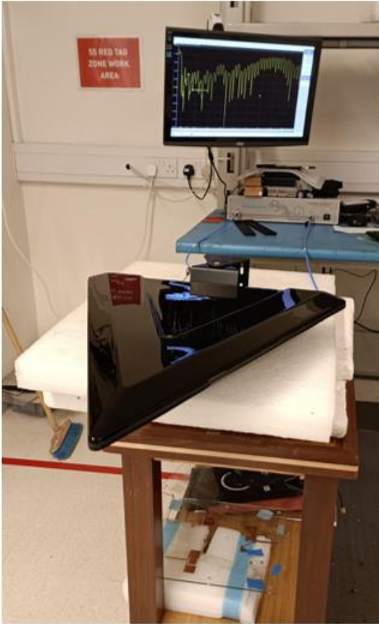
VNA Setup
