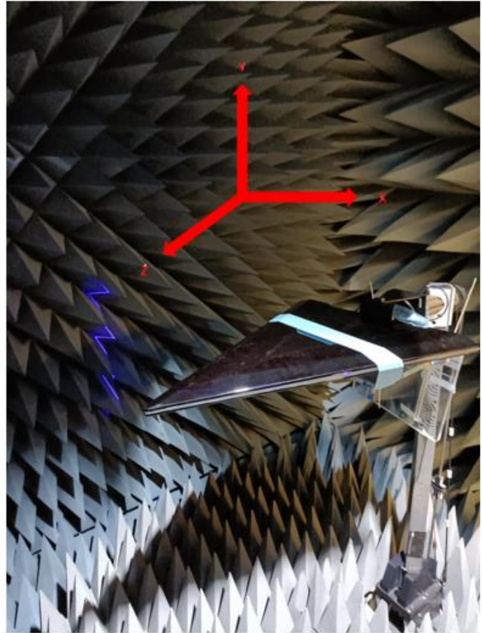
Anechoic Chamber Setup
