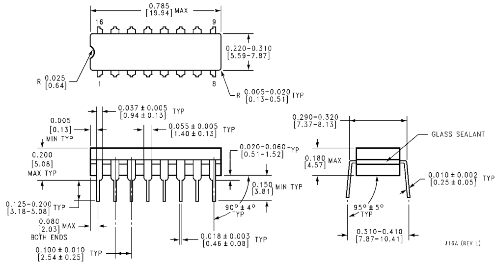
16-Lead Ceramic Dual-In-Line Package (J) Order Number 54LS365ADMQB or DM54LS365AJ Package Number J16A
