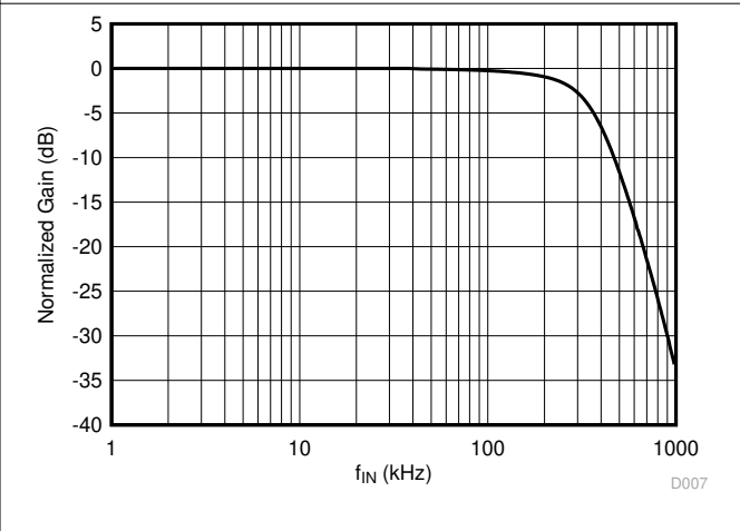
Figure 6-20. Normalized Gain vs Input Frequency
