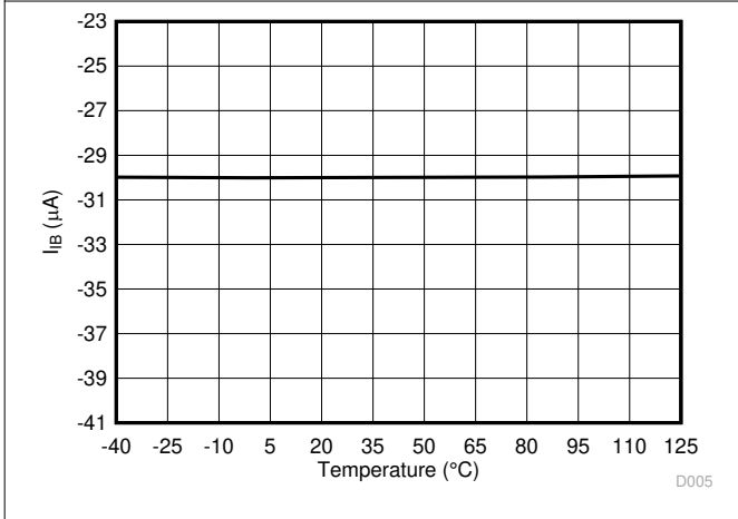
Figure 6-15. Input Bias Current vs Temperature
