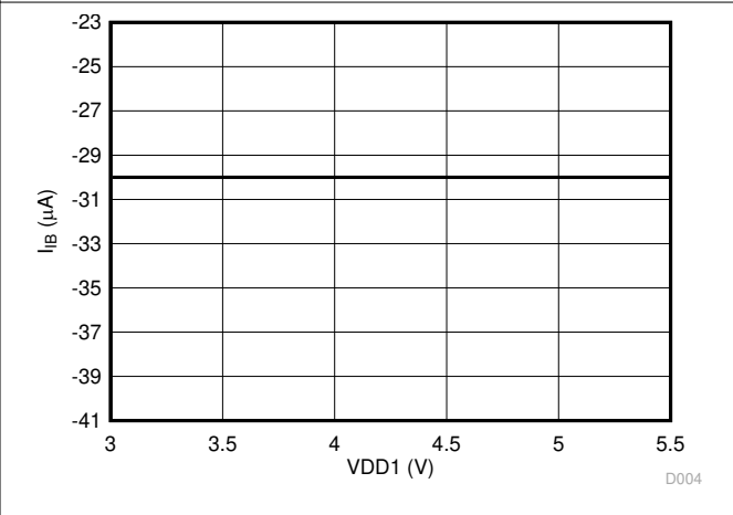
Figure 6-14. Input Bias Current vs High-Side Supply Voltage
