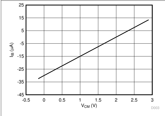
Figure 6-13. Input Bias Current vs Common-Mode Input Voltage
