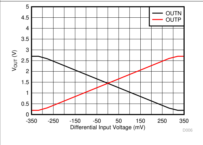
Figure 6-22. Output Voltage vs Input Voltage
