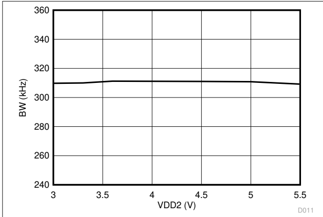
Figure 6-35. Output Bandwidth vs Low-Side Supply Voltage
