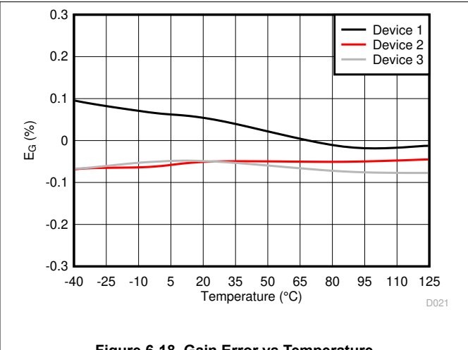
Figure 6-18. Gain Error vs Temperature
