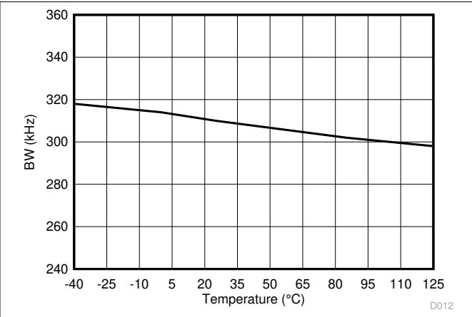
Figure 6-36. Output Bandwidth vs Temperature
