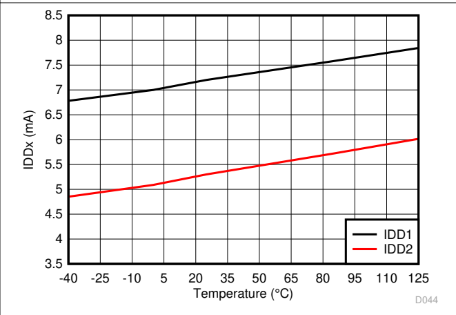
Figure 6-38. Supply Current vs Temperature
