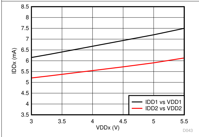
Figure 6-37. Supply Current vs Supply Voltage
