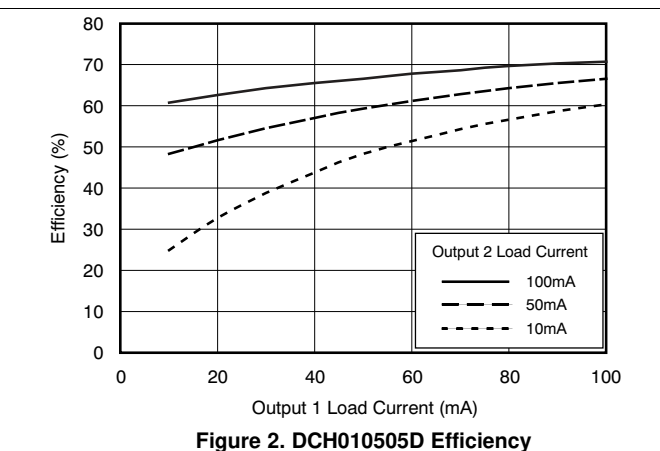
Figure 2. DCH010505D Efficiency
