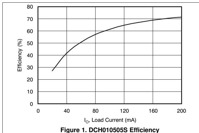
Figure 1. DCH010505S Efficiency
