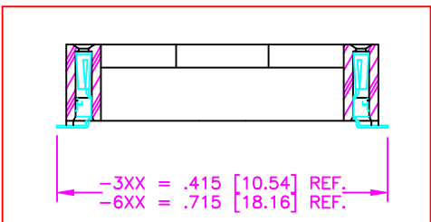
FIG. 2 LEAD STYLE 0 SAME AS FIG 1 EXCEPT AS SHOWN
