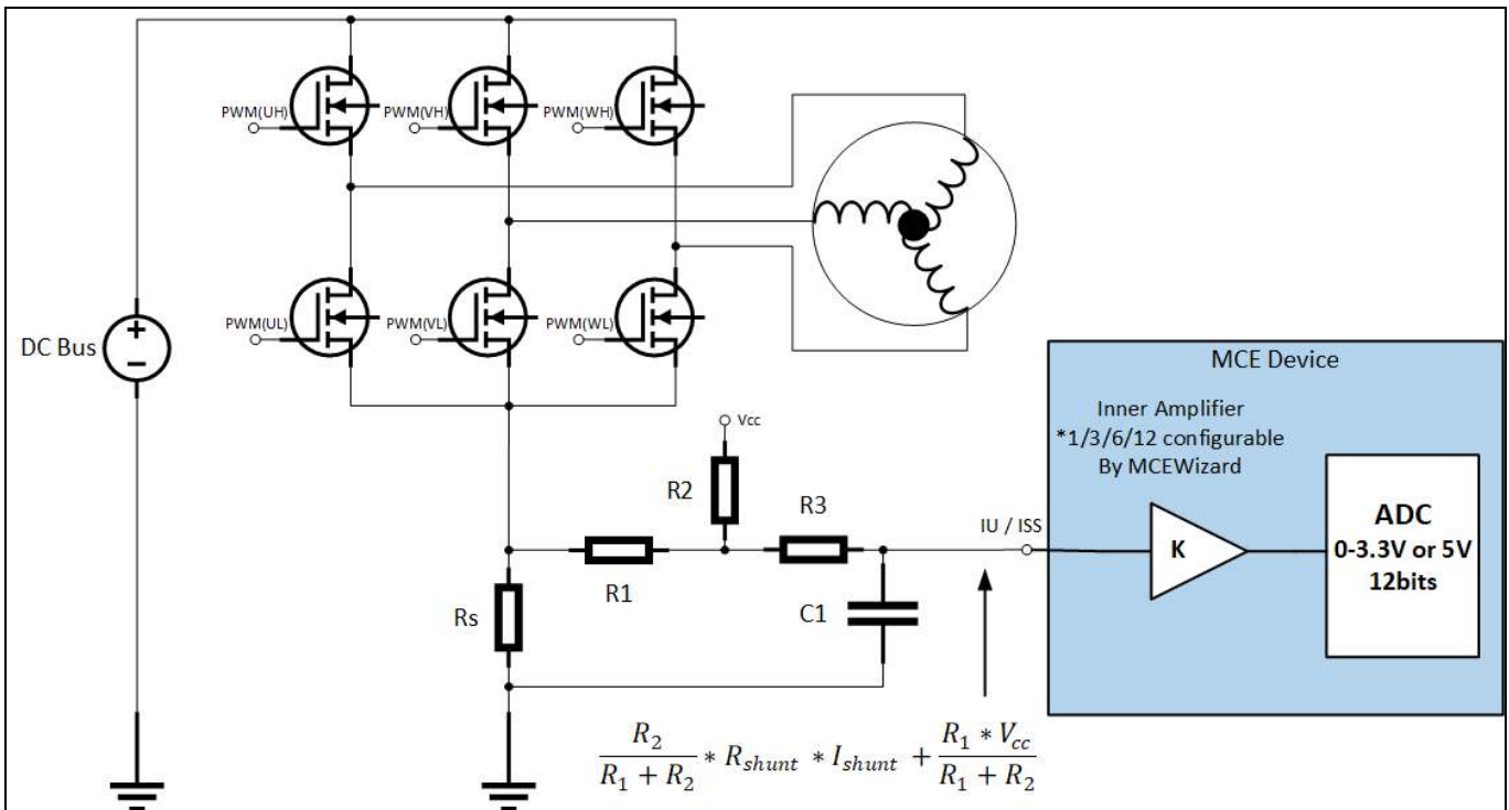
Figure 14 Current-sensing topology
