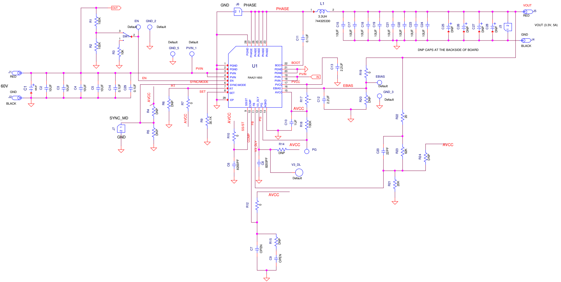
Figure 4. RTKA211650DE0000BU Schematic
