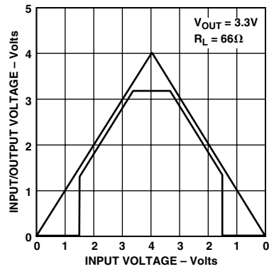
TPC 8. Power-Up/Power-Down
