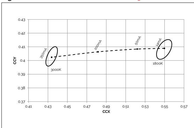
Figure 8: Color shift vs. Forward Current 3000K - 1800K
