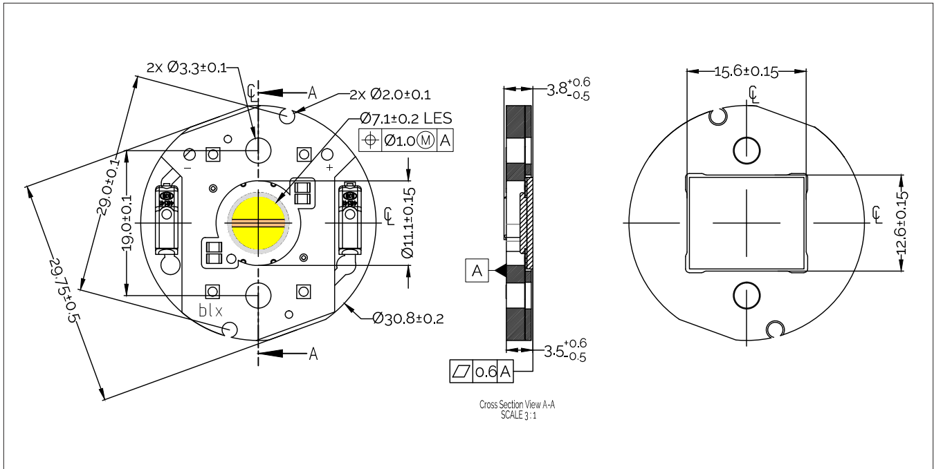
Figure 12: Mechanical Drawing Specifications
