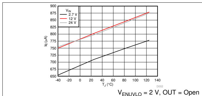
Figure 8. Quiescent Current vs Temperature
