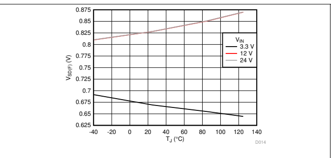
Figure 9. EN/UVLO Falling Threshold for Lowest Current Consumption
