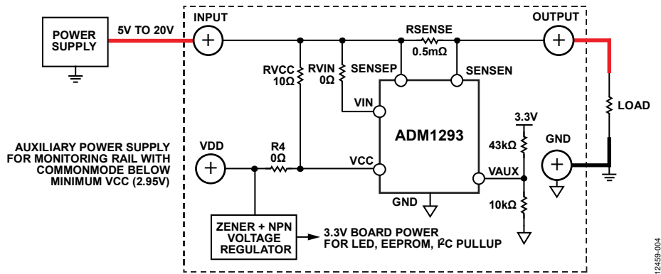
Figure 3. Power Supply And Load Connection For ADM1293 Evaluation Board
