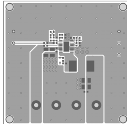
Figure 2 – Top Layer
