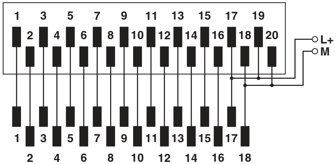
Circuit diagram
