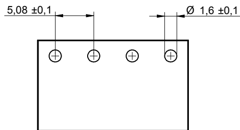
RECOMMENDED PCB LAYOUT - COMPONENT VIEW
