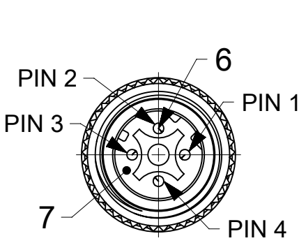
VIEW FROM THE FRONT SIDE RJ45 HIDDEN FOR CLARITY SCALE 2:1
