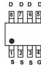
pin assignment
