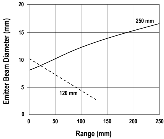
Figure 10. Typical emitter spot diameter vs. distance for AF250 and AF120
