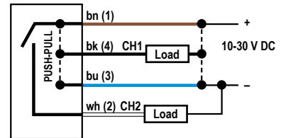
Figure 4. IO-Link with PNP output
