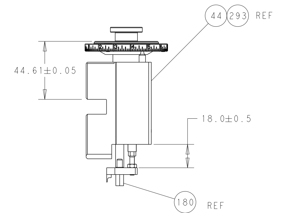
RAM & HOLD DOWN SET-UP
