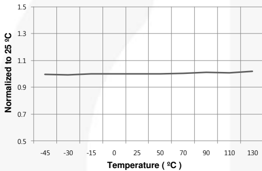
Figure 13. V_{VS-SLP-TH} vs. Temperature
