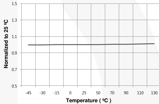
Figure 14. V_{VS-OVP} vs. Temperature
