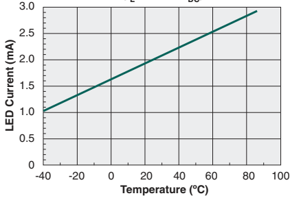
Typical I_F for Switch Operation vs. Temperature ( I_L=200\text{mA}_{DC} )
