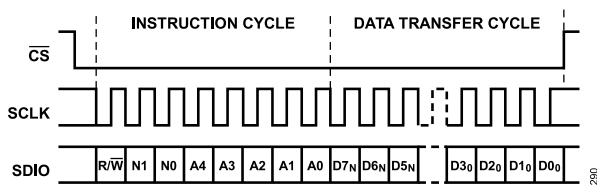
Figure 86. Serial Register Interface Timing, MSB First Read
