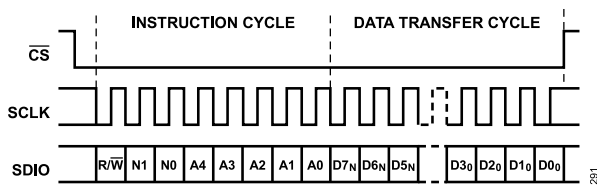
Figure 85. Serial Register Interface Timing, MSB First Write
