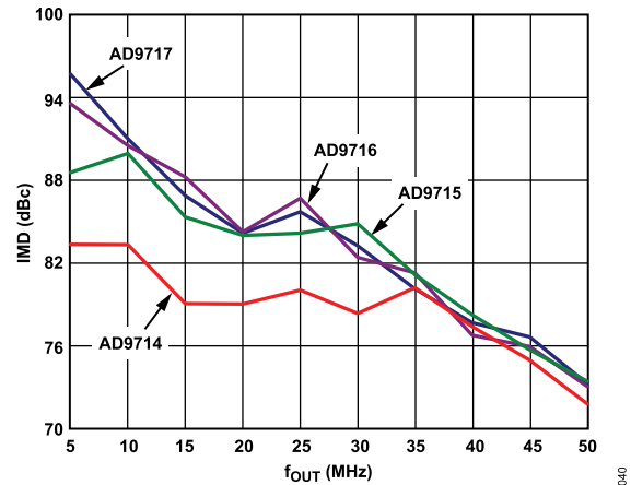
Figure 47. AD9714/AD9715/AD9716/AD9717 IMD at 3.3 V
