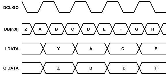
Figure 92. Timing Diagram with IFIRST = 1, IRISING = 1
