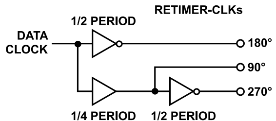
Figure 95. RETIMER-CLK Phases
