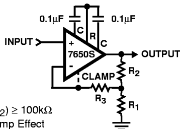
FIGURE 2. NON INVERTING AMPLIFIER WITH OPTIONAL
