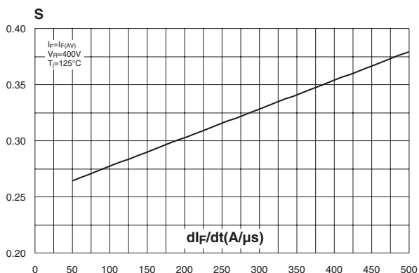
Fig. 7: Reverse recovery softness factor versus di_F/dt (typical values).
