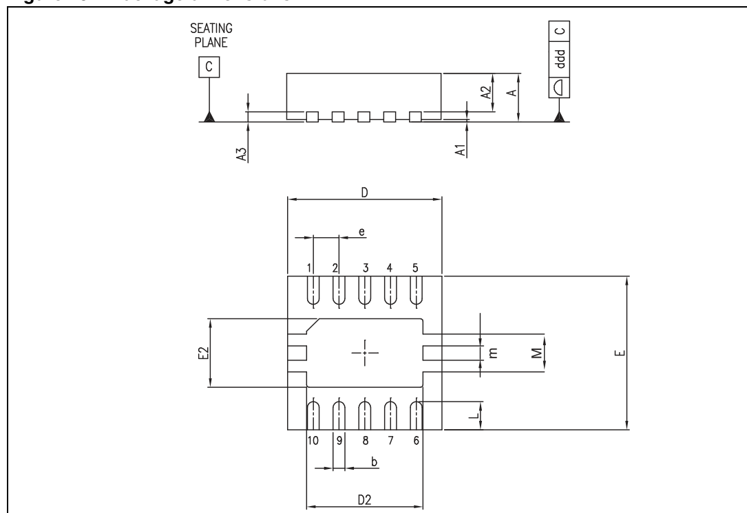
Figure 10. Package dimensions
