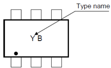
Fig. 9.2 Marking RN2902FE
